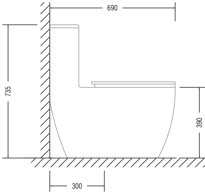
SIDE VIEW
